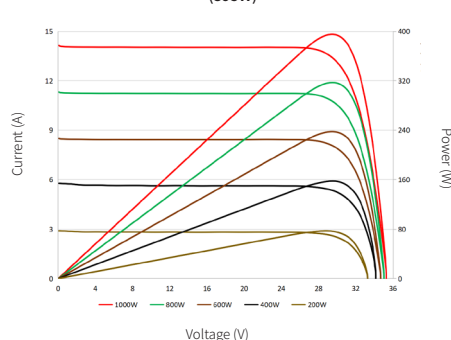
Current-Voltage &amp; Power-Voltage Curves (395W)
